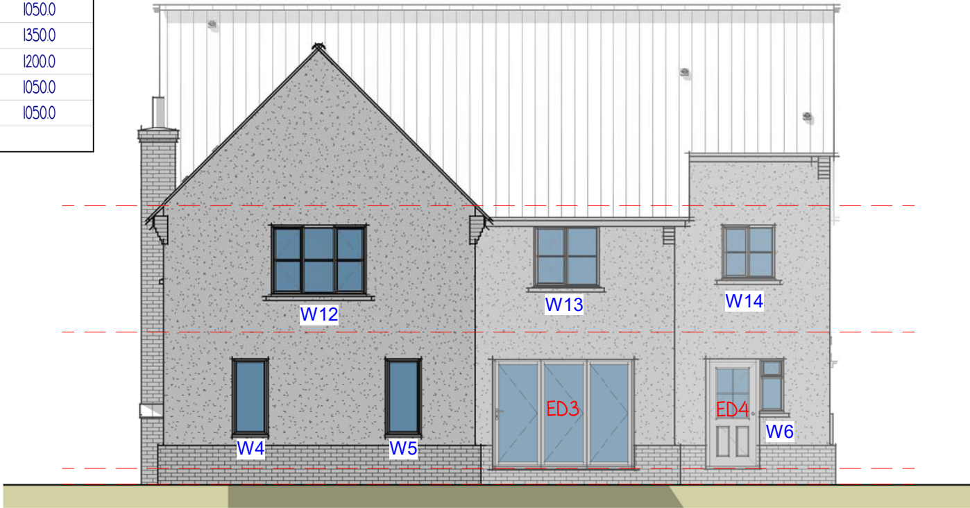
Elevation 03 - Rear 1 : 100
