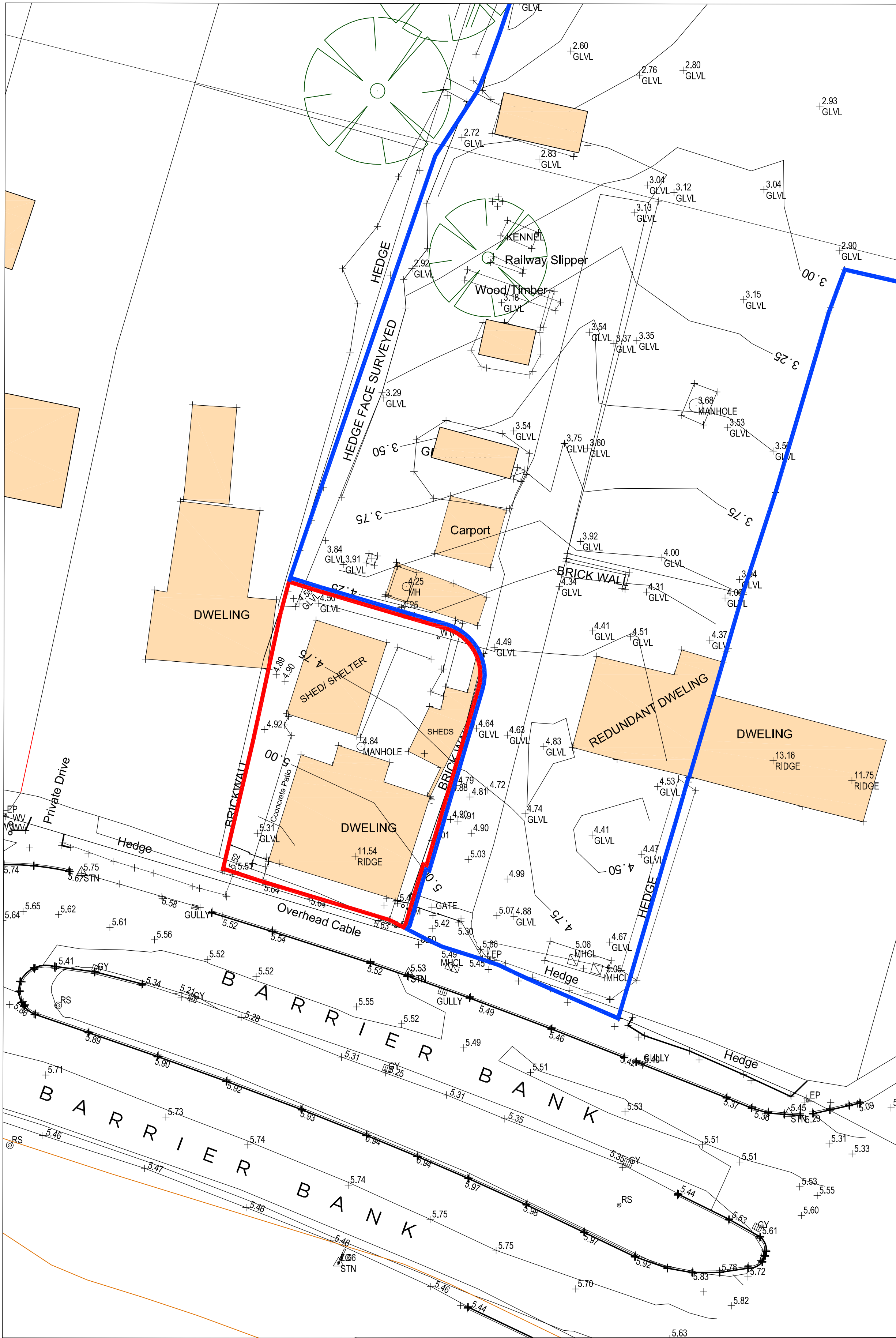
Existing Site Layout Scale 1:200
