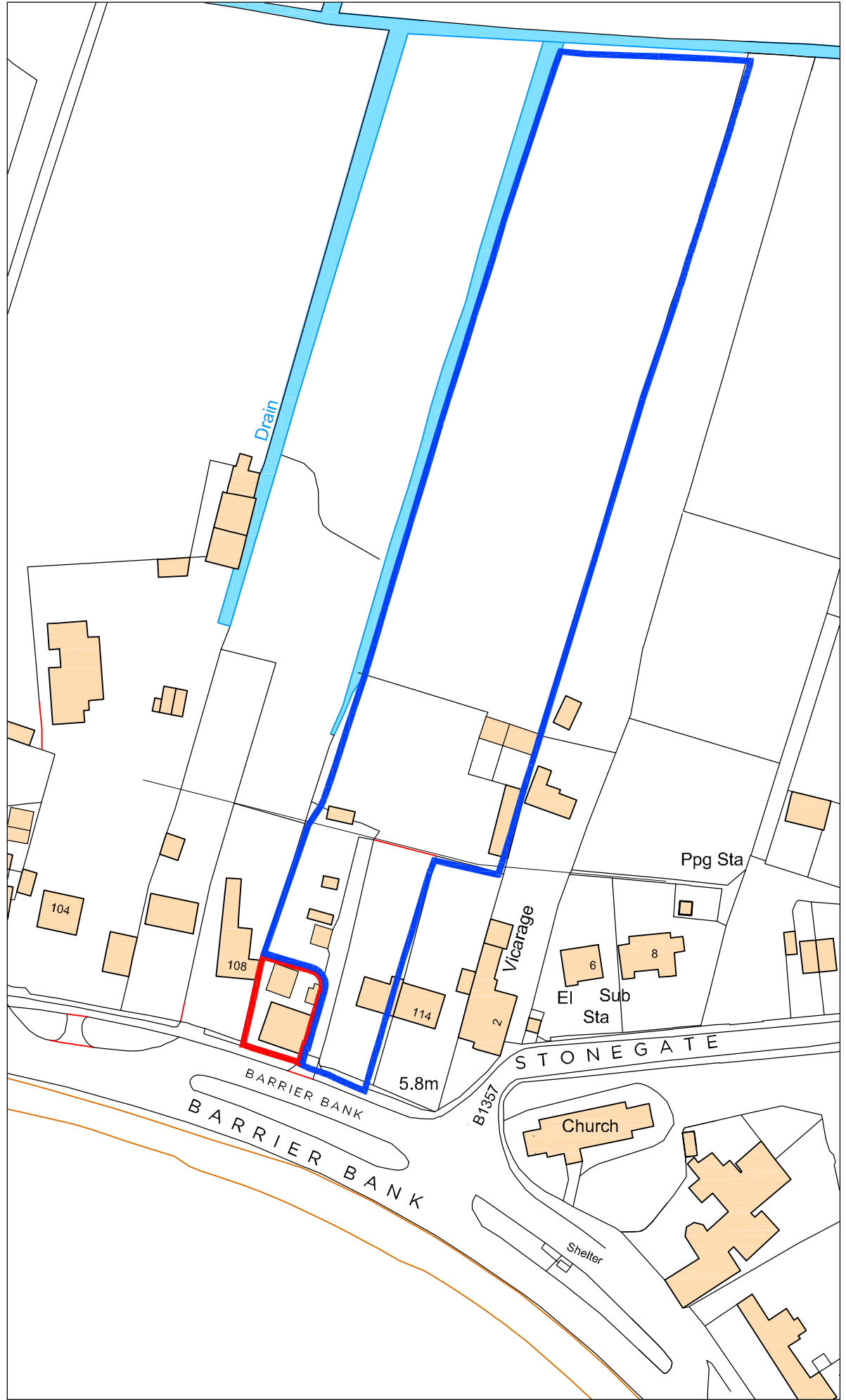
Site Location Plan Scale 1:1250
