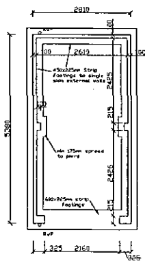
FOUNDATION PLAN
