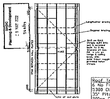
TRUSS LAYOUT
