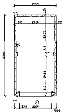
FLOOR PLAN
