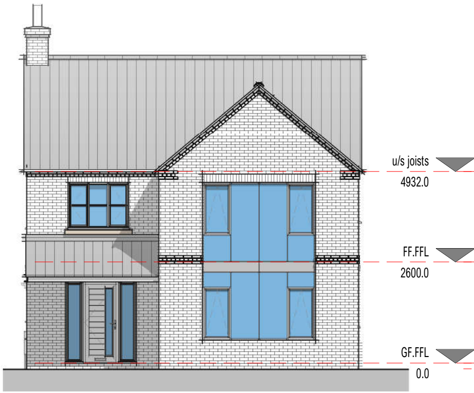
Elevation 01 - Front
