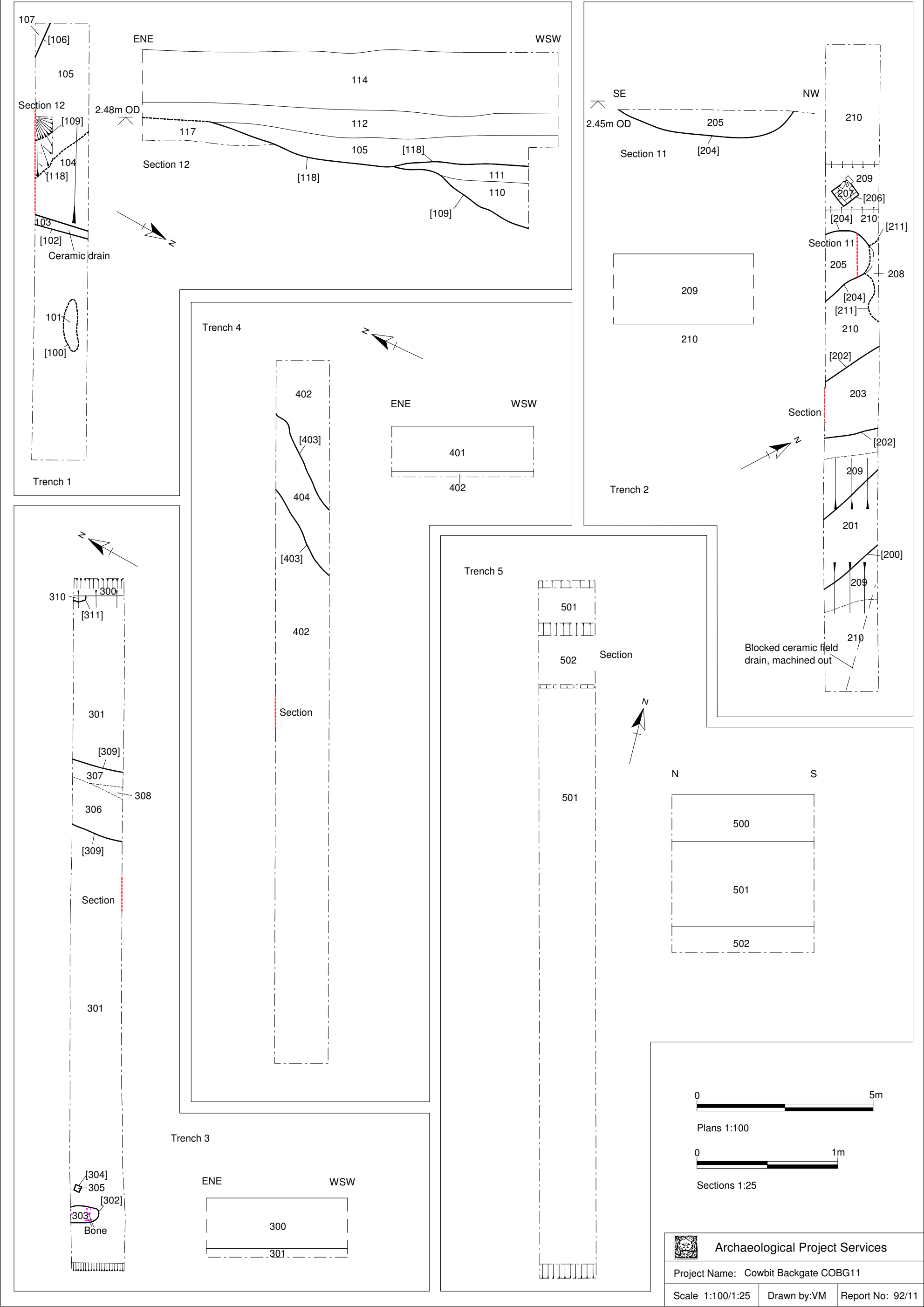
Figure 4 Plans and sections, Trenches 1-5
