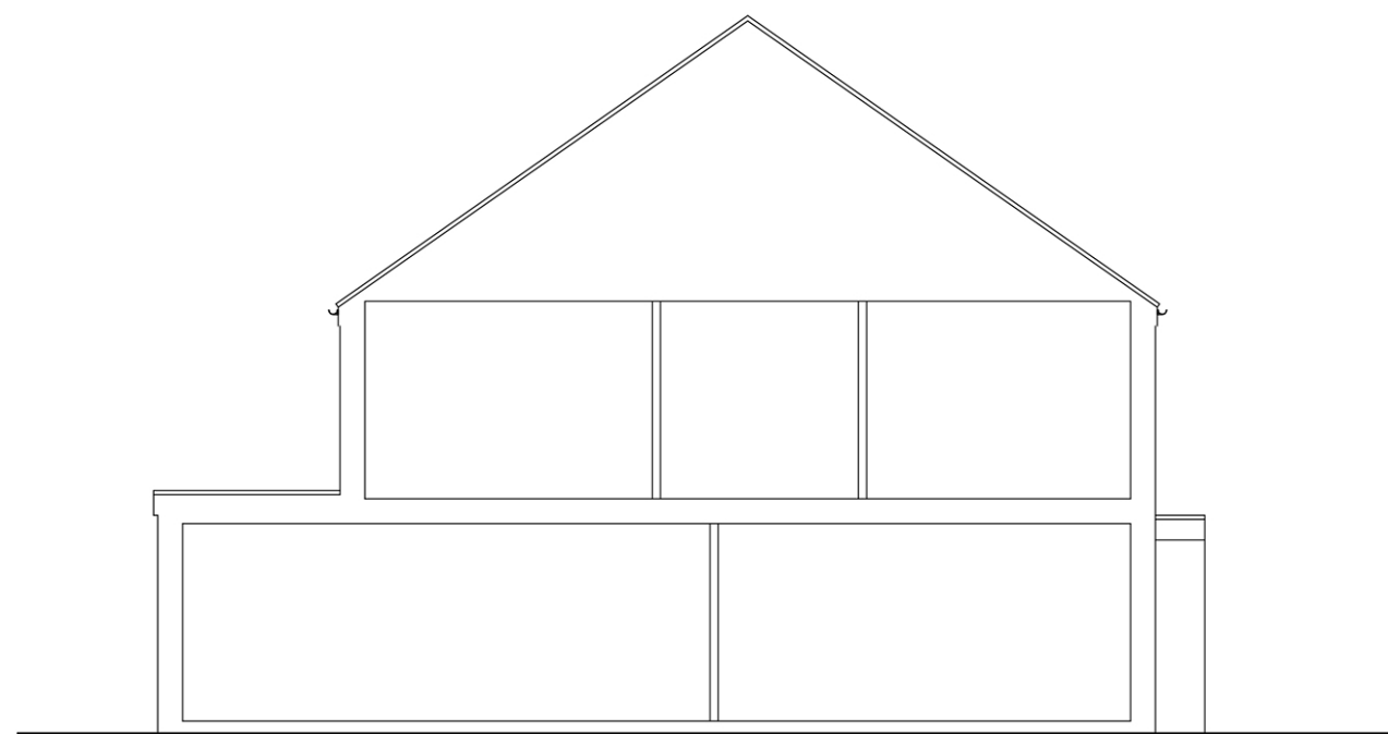
Section 1:100
