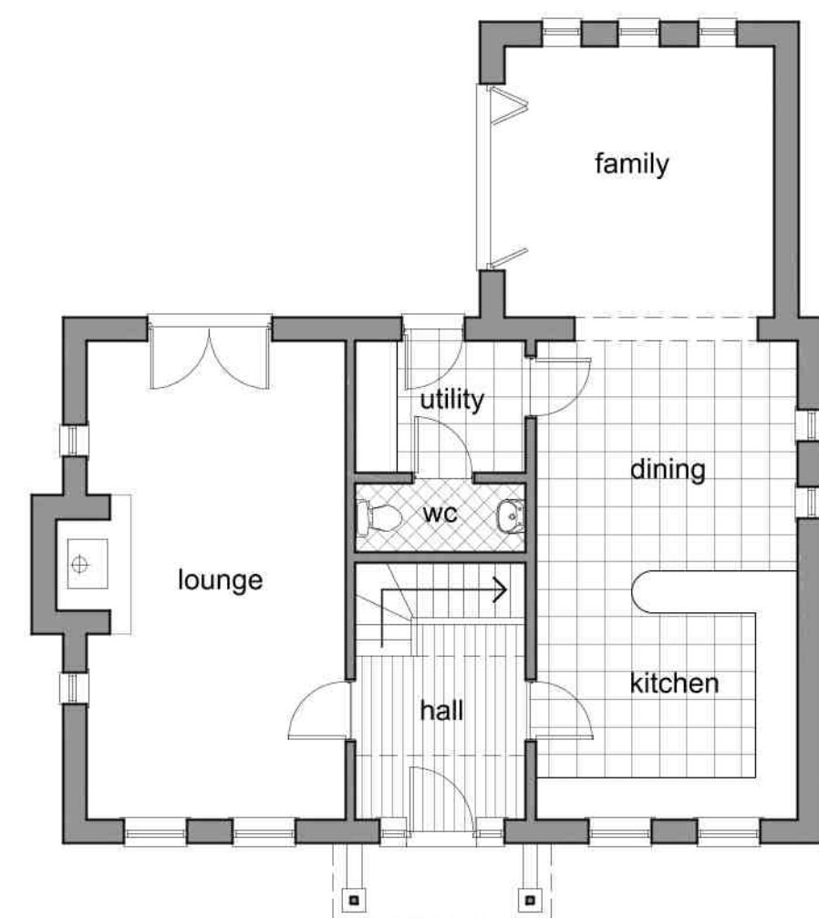
Indicative Ground Floor Plan
