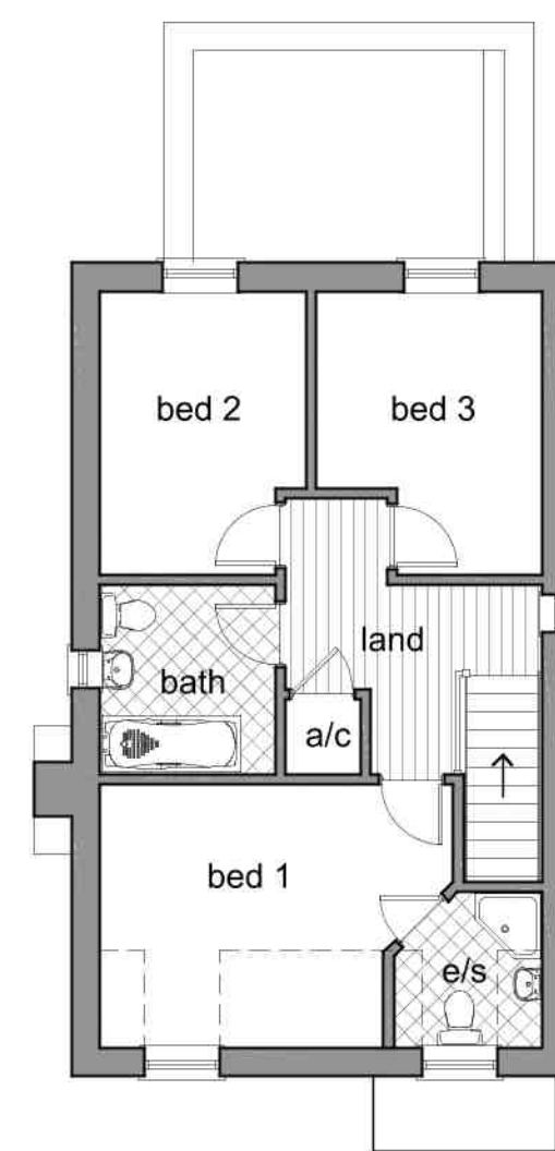
Indicative First Floor Plan
