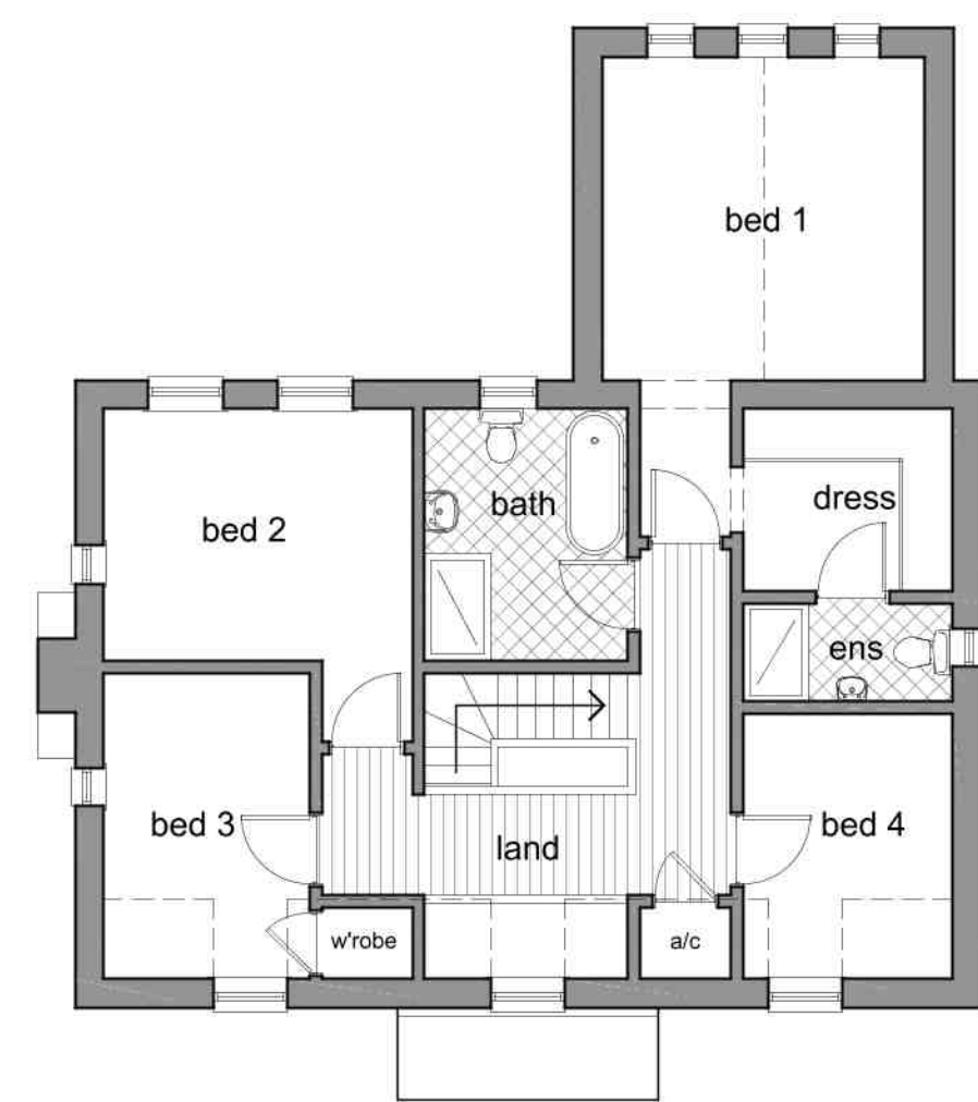
Indicative First Floor Plan
