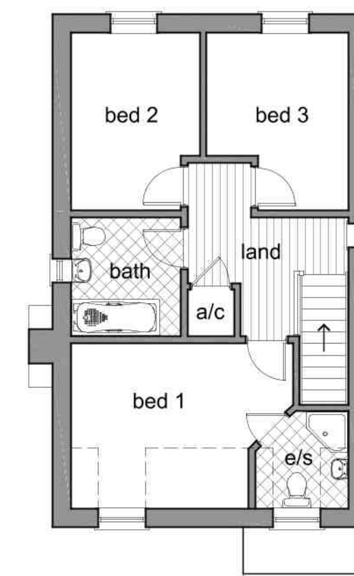
Indicative First Floor Plan
