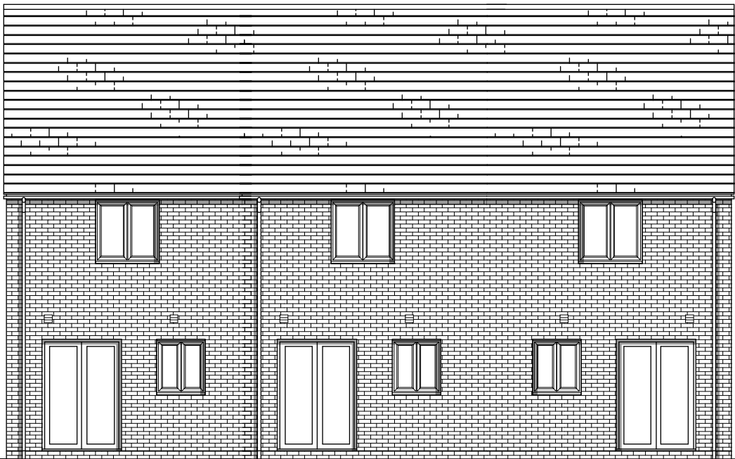
REAR ELEVATION
