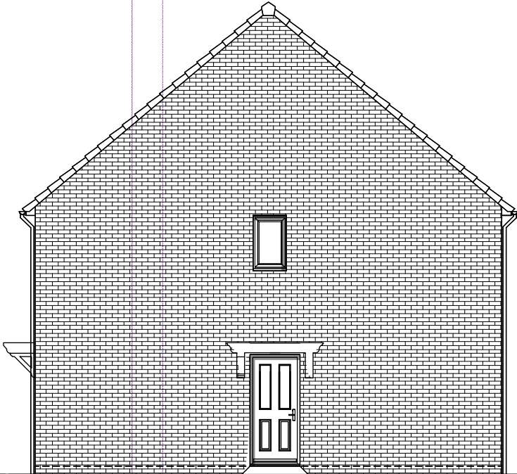
SIDE ELEVATION
