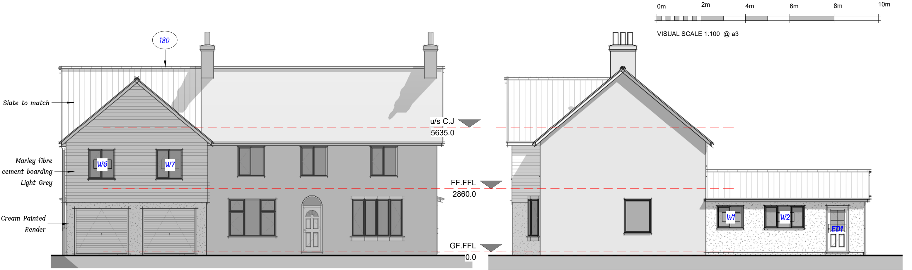
Elevation 01 - Front
