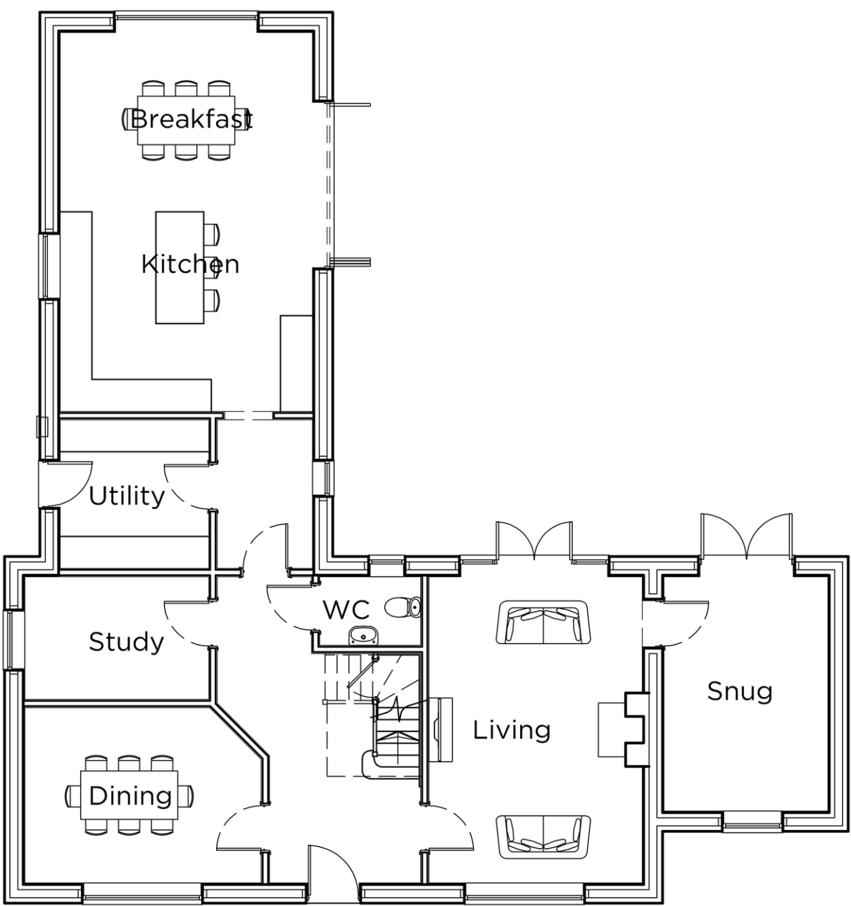
Ground Floor
