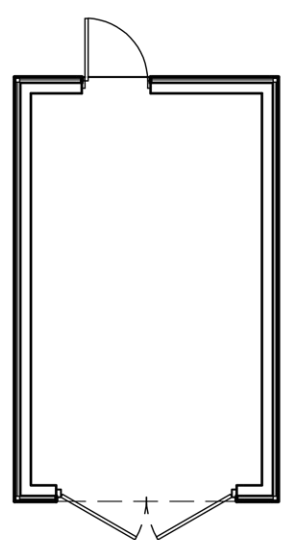
Plot 1 Oak Framed Store Floor Plan
