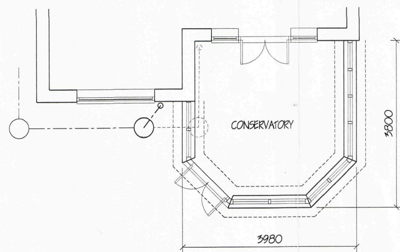
FLOOR PLAN
