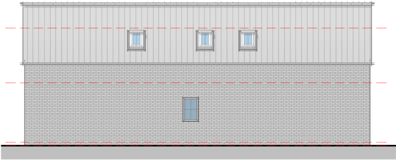
Elevation 03 - Rear 1 : 100
