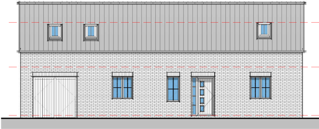
Elevation 01 - Front 1 : 100
