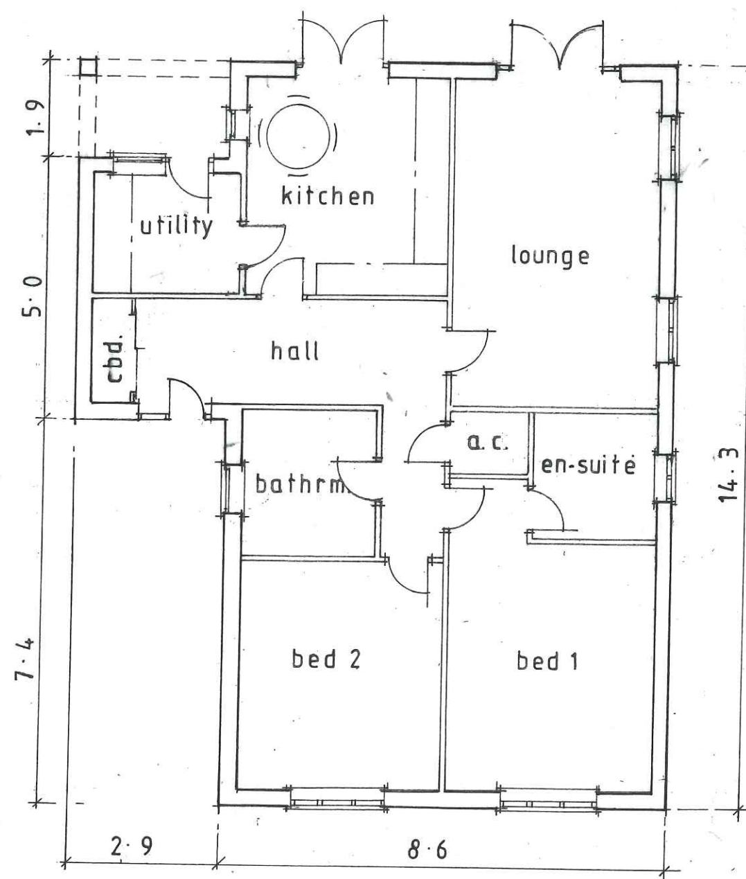
PROPOSED LAYOUT 1:100
