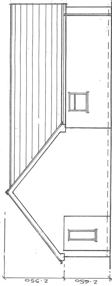
PROPOSED SIDE ELEVATION 1:100
