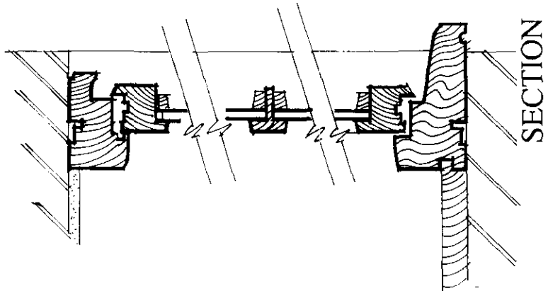
TYPICAL WINDOW HORIZONTAL BAR CASEMENT CREAM PAINTED TIMBER
