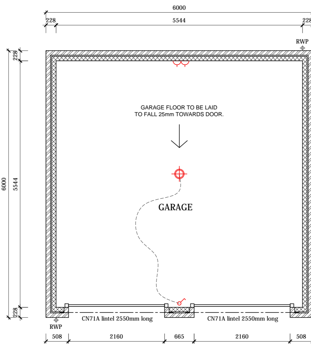
GARAGE PLAN
