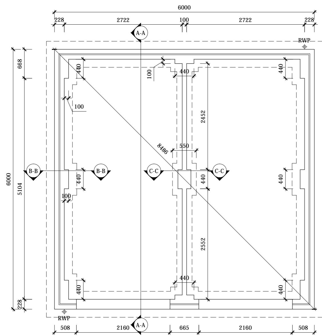
SUBSTRUCTURE PLAN
