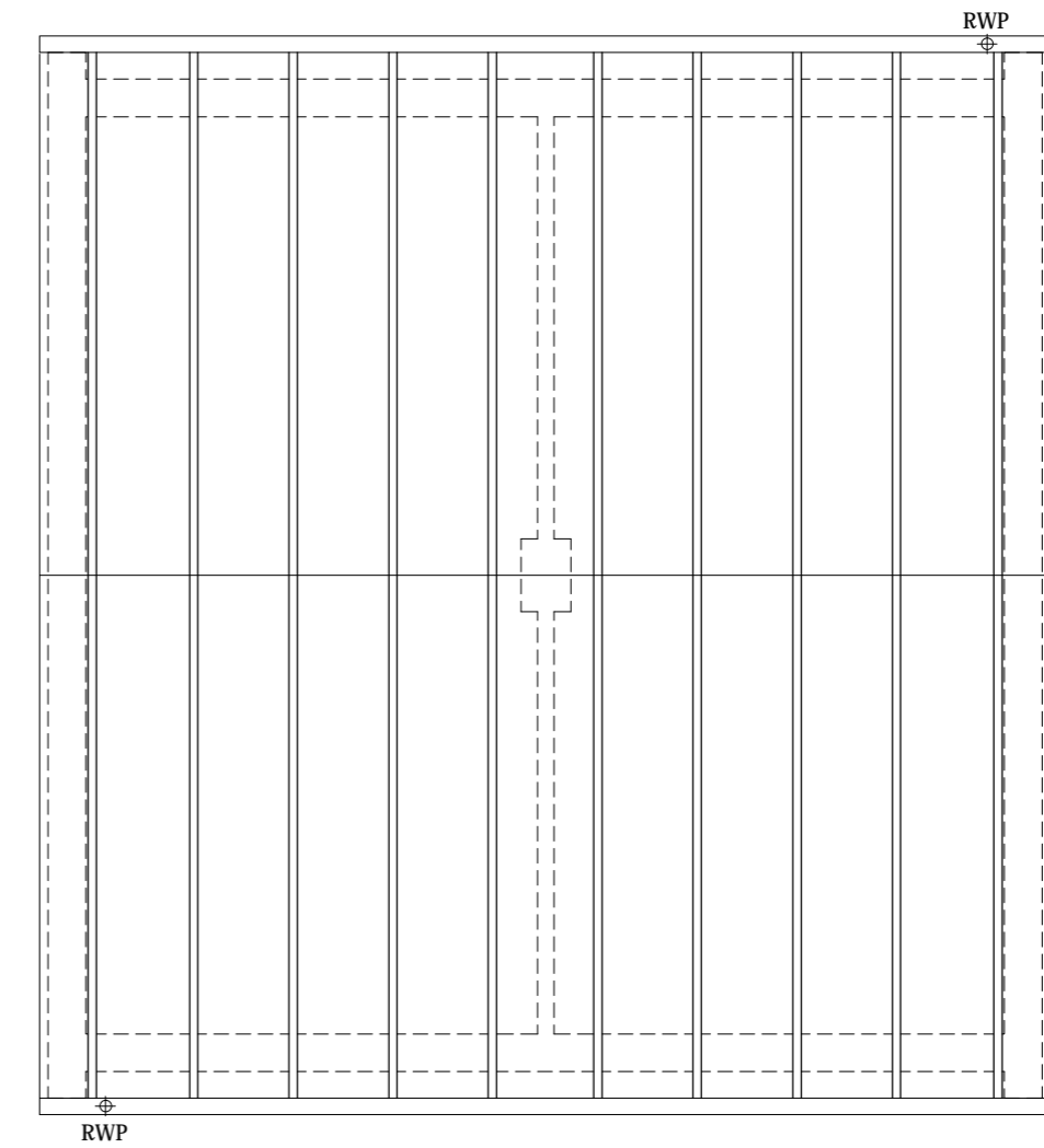
ROOF PLAN PITCH 35°
