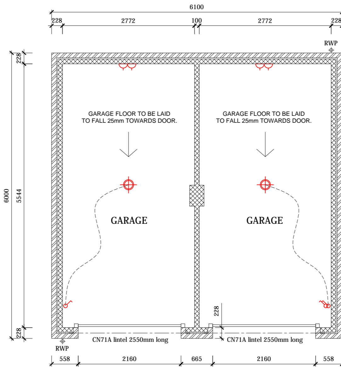
GARAGE PLAN
