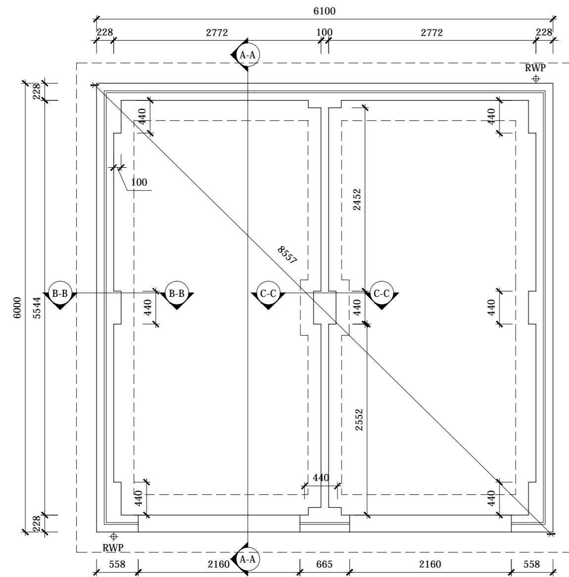
SUBSTRUCTURE PLAN
