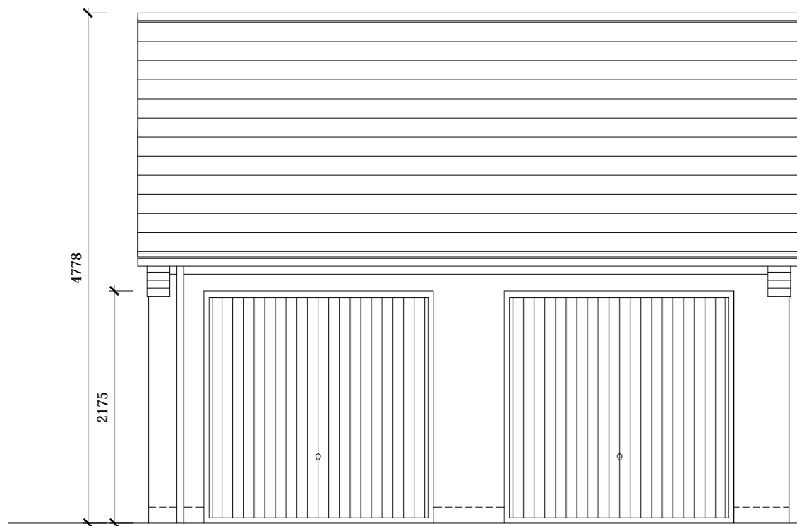
FRONT ELEVATION
