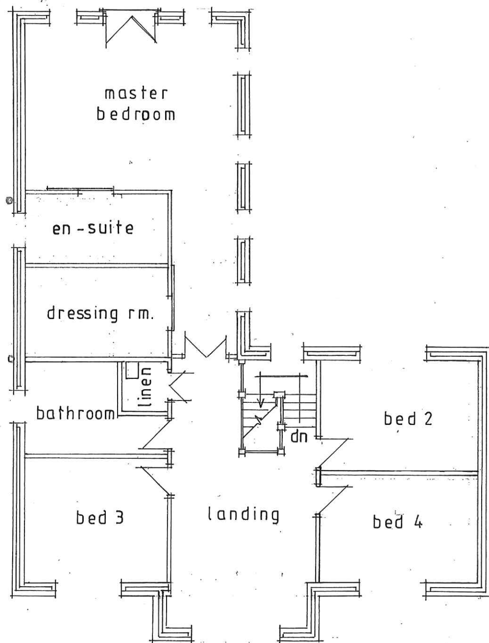
FIRST FLOOR LAYOUT 1:100
