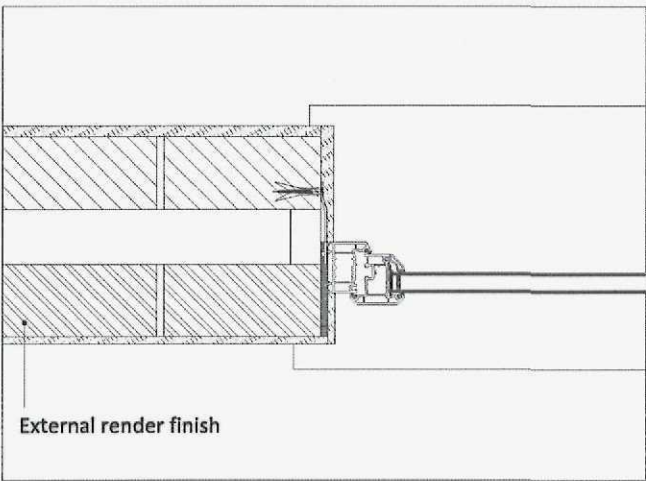
WINDOW JAMB SECTION
