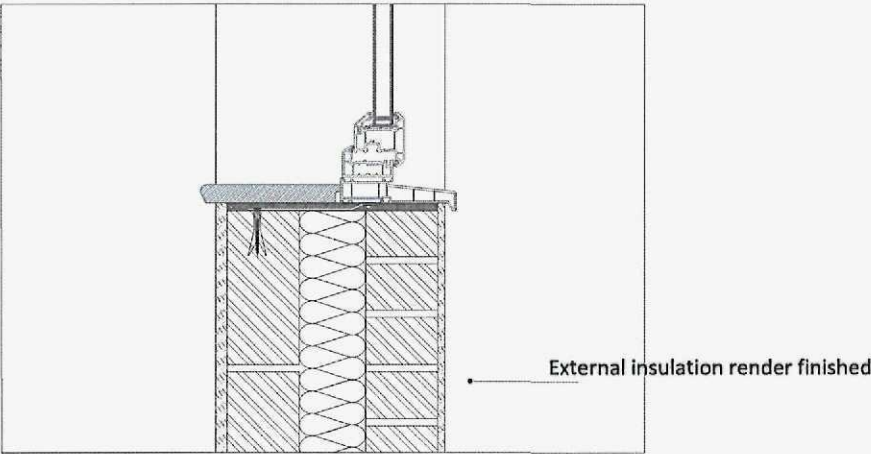
WINDOW CILL SECTION
