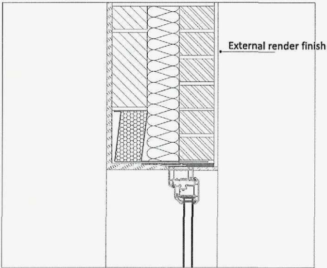
WINDOW HEAD SECTION
