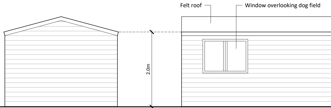
West elevation
