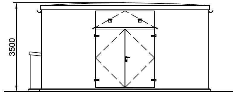
Elevation A 1:100
