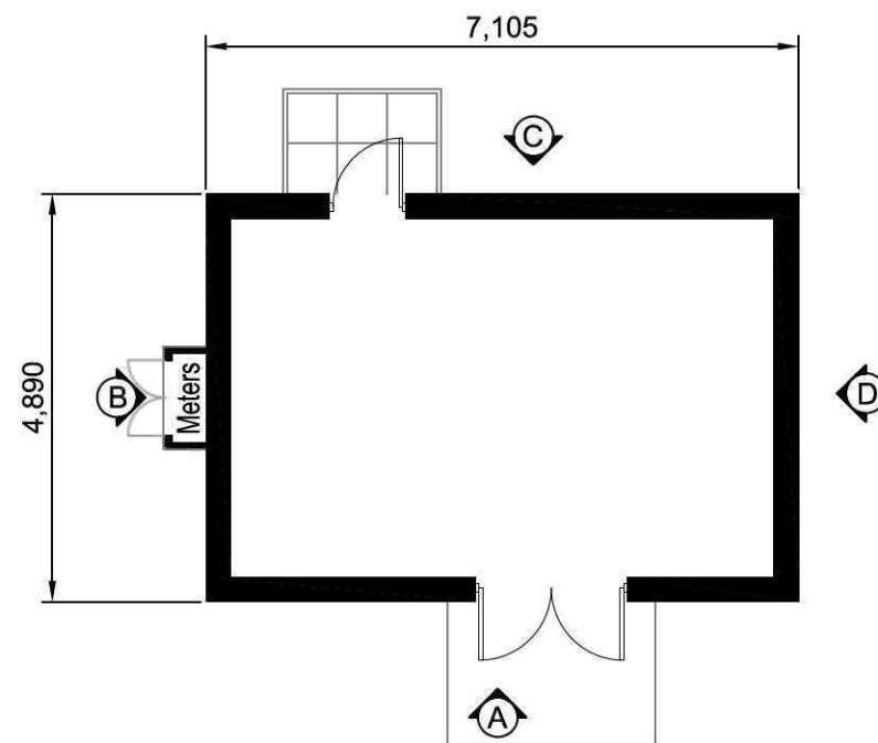
Typical DNO 33kV GRP Switchroom Plan 1:100
