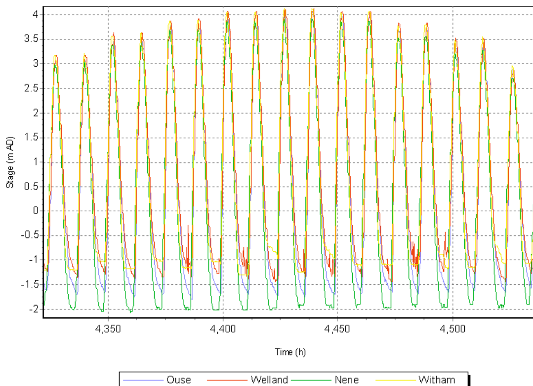
Figure 2-3: Sample period from the tide series at the four outfalls
