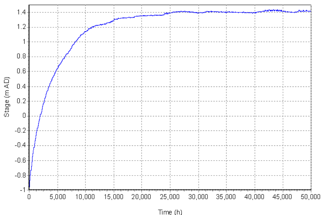
Figure 2-4: Results of the water-balance model run: water level in the Fens
