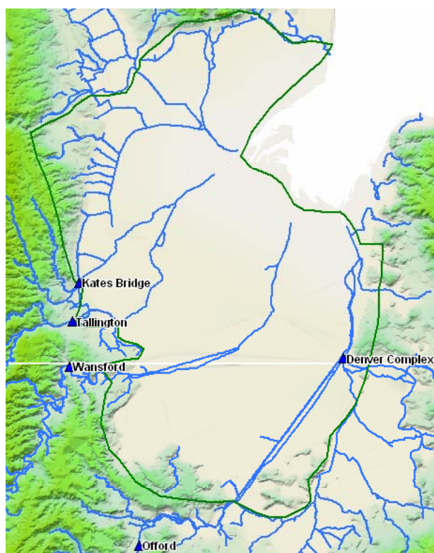
Figure 3-4 Location of flow gauges used in analysis
