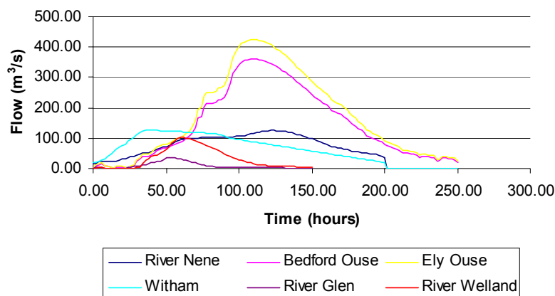
Figure 3-1 Hydrographs resulting in 1% water levels in the Fens
