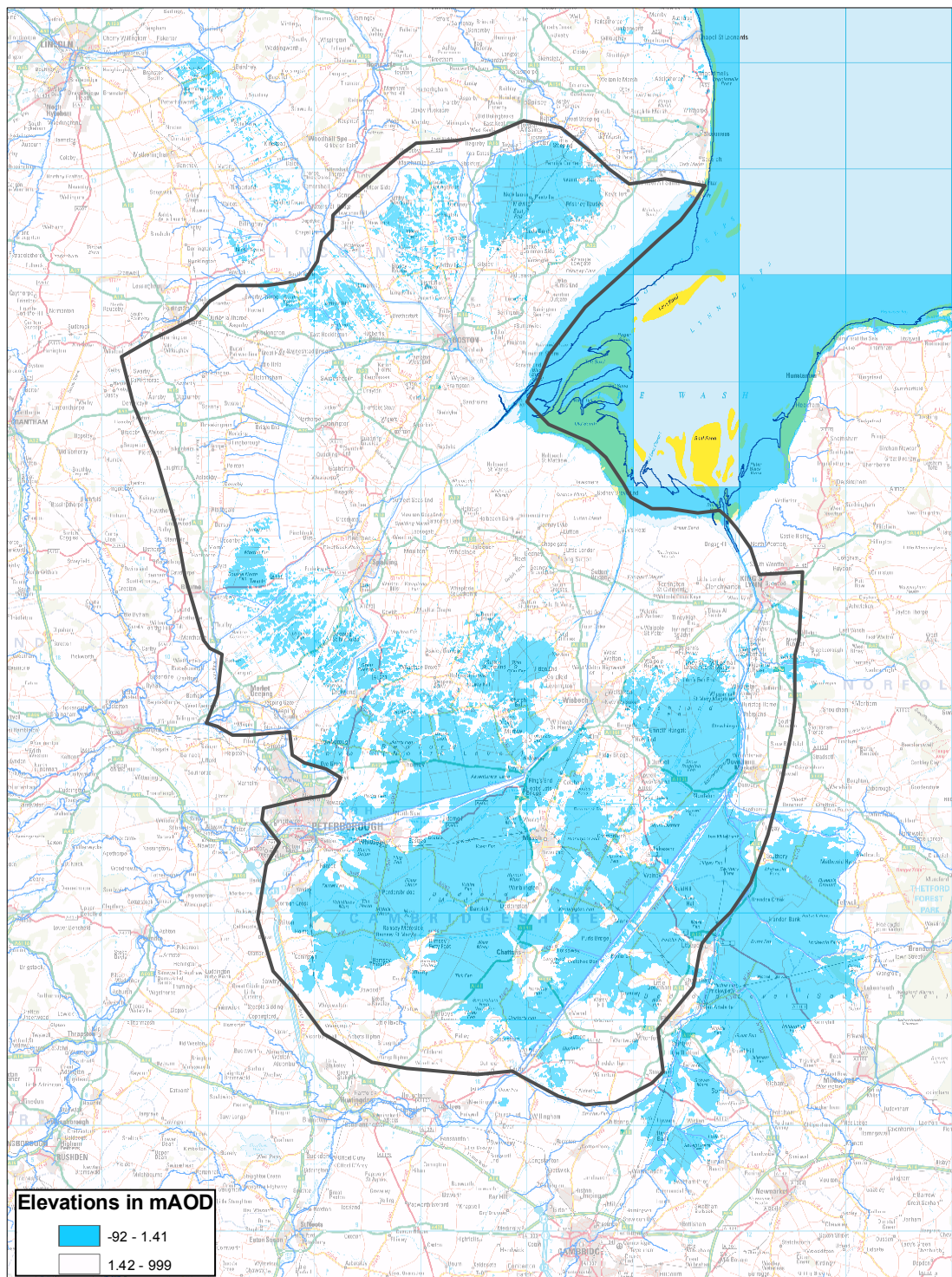
Figure 2-5: Area below 1.42m AOD (flooded in equilibrium model)
