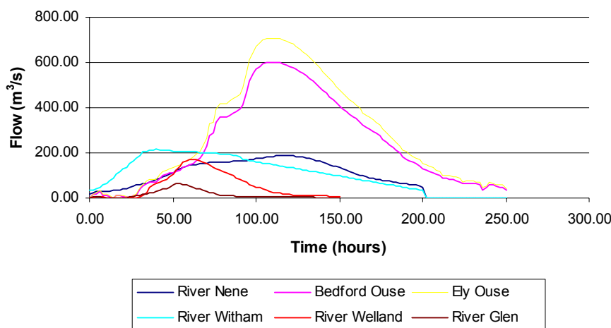
Figure 3-2 Hydrographs resulting in 0.1% water levels in the Fens
