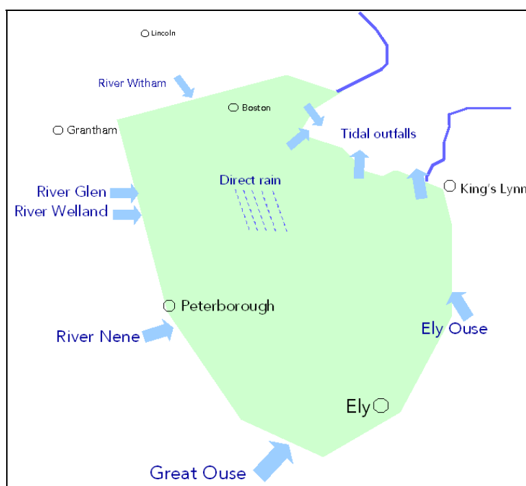
Figure 2-2: Conceptual model of Fens for simulating equilibrium level
