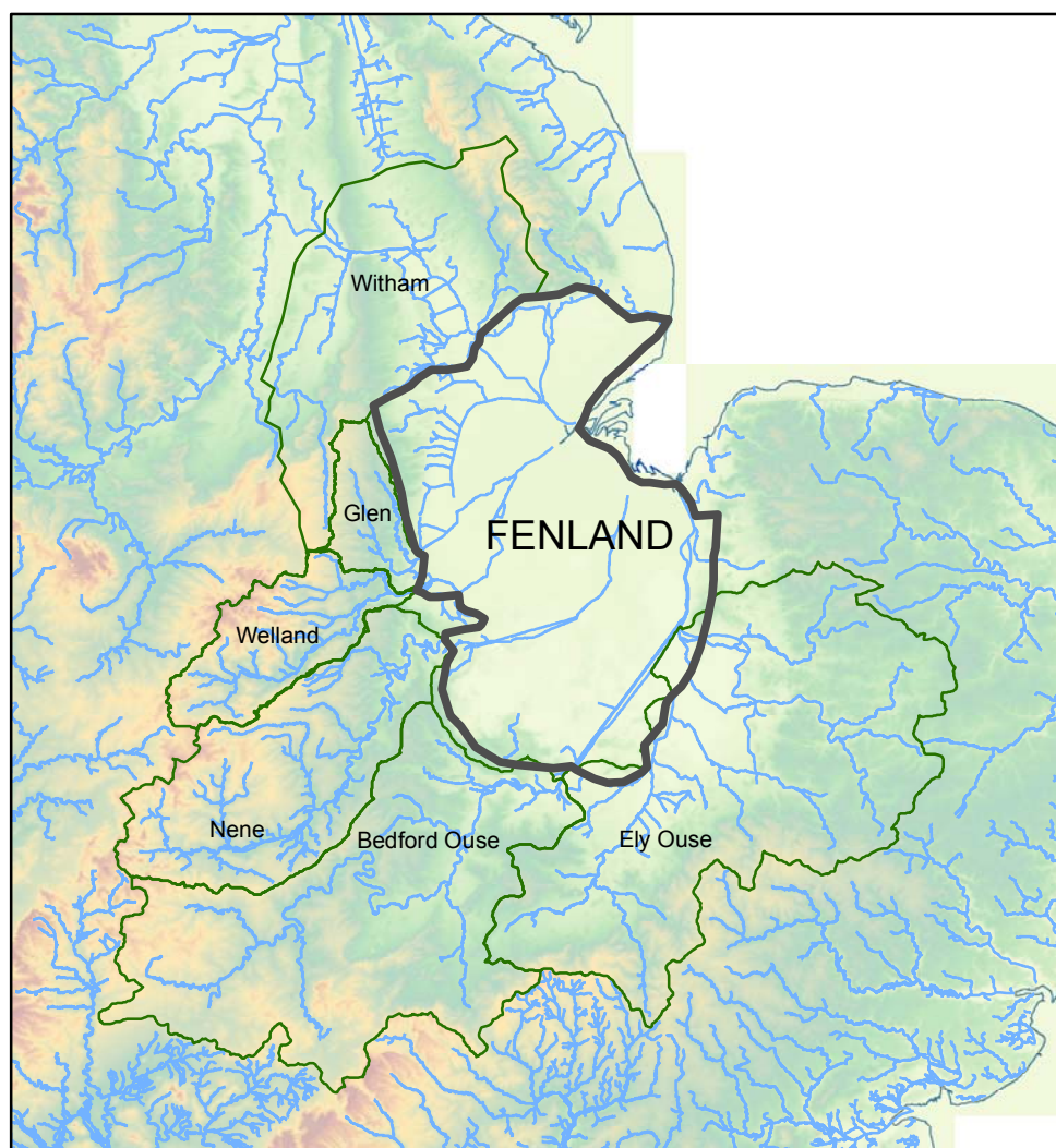
Figure 2-1: Main catchments draining to the Fens
