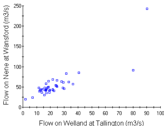
Figure 3-3 Correlation between peak flows on Rivers Nene and Welland
