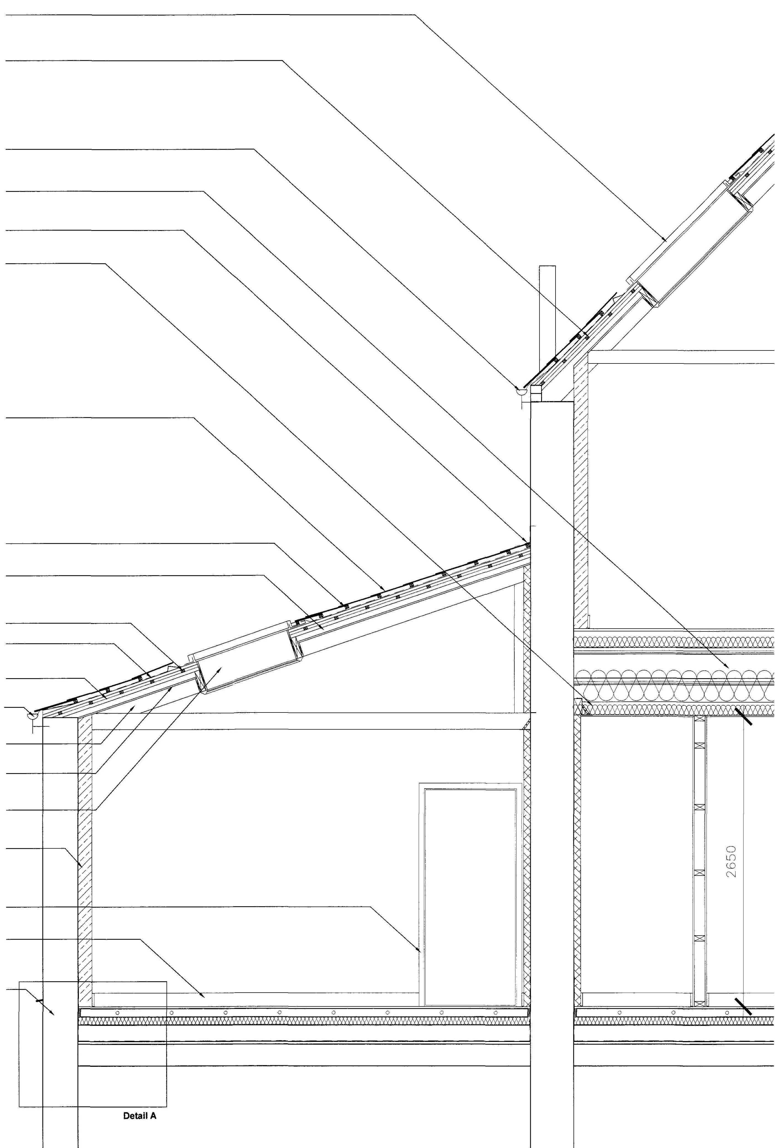
Proposed Section
