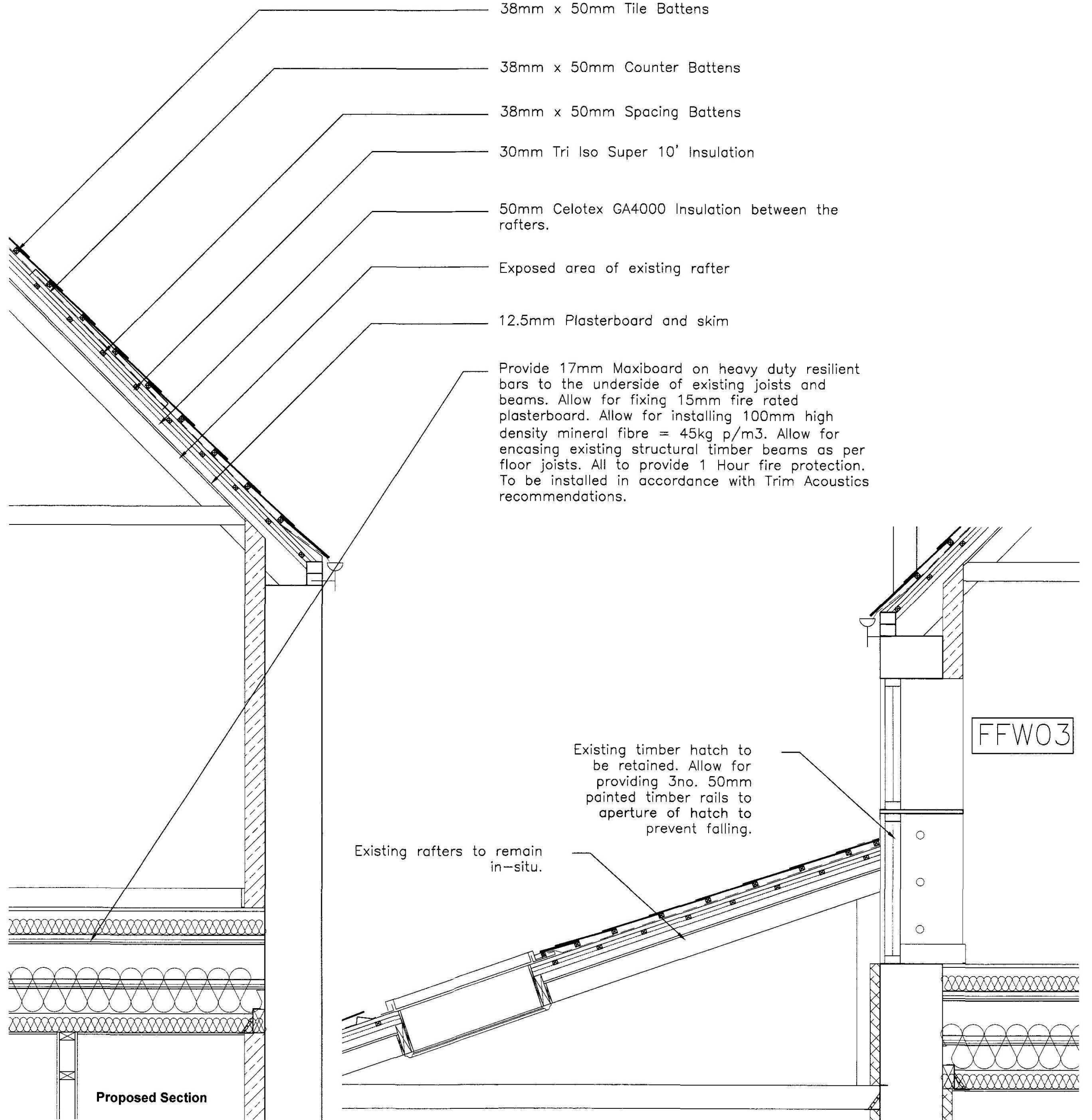
Proposed Section through hatch
