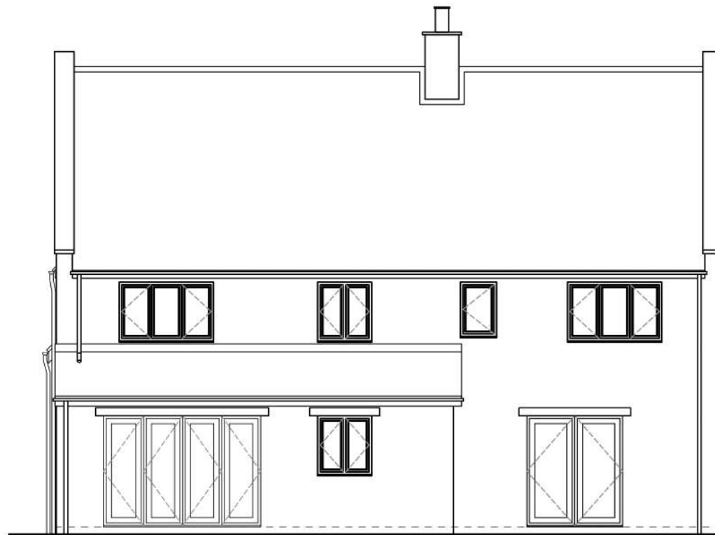
Rear Elevation
