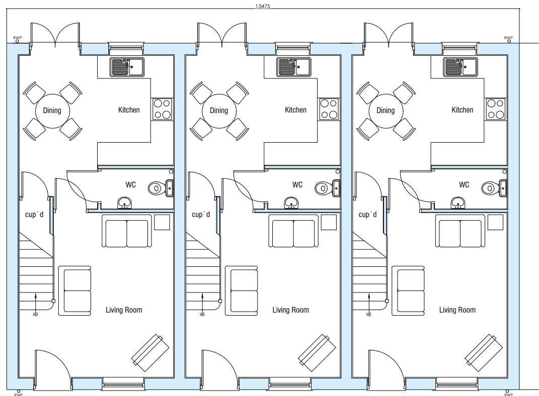
Ground Floor Plan Total Floor Area - 69.94 m 2 / 752.84 ft 2 Plots 1, 2 & 3.
