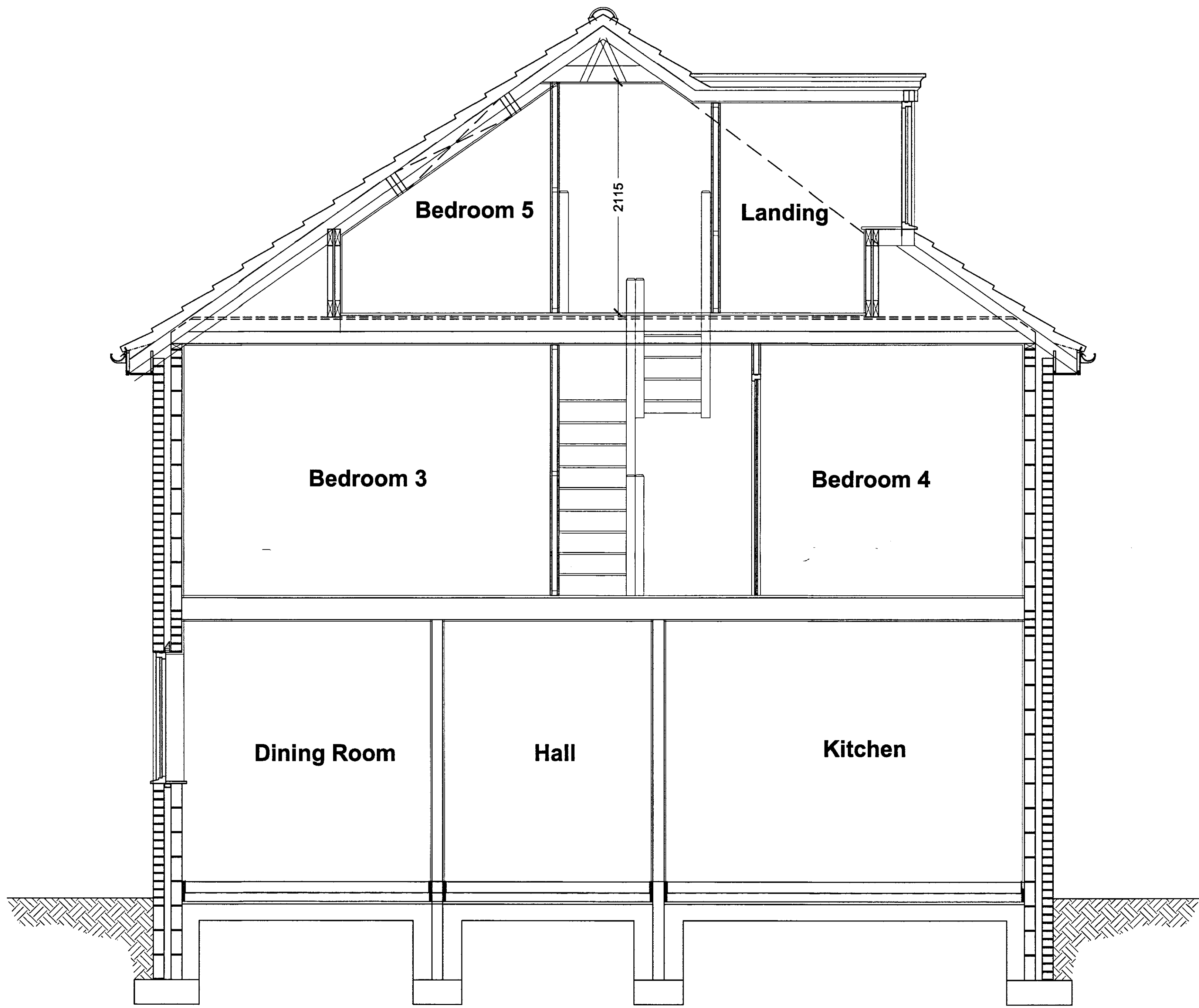
Proposed Section A-A Scale 1:25
