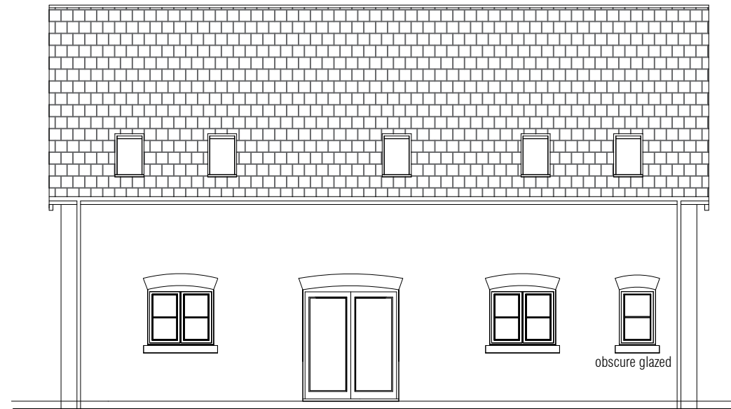
rear elevation - plots 2 & 3
