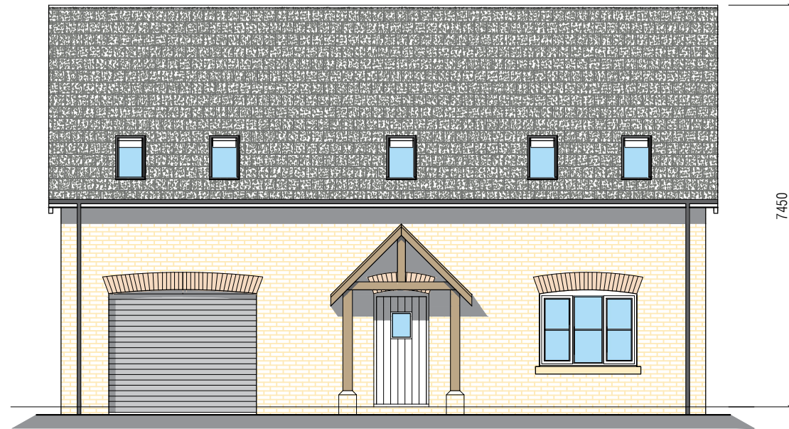
front elevation - plots 2 & 3
