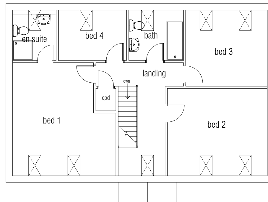
first floor layout - plots 2 & 3
