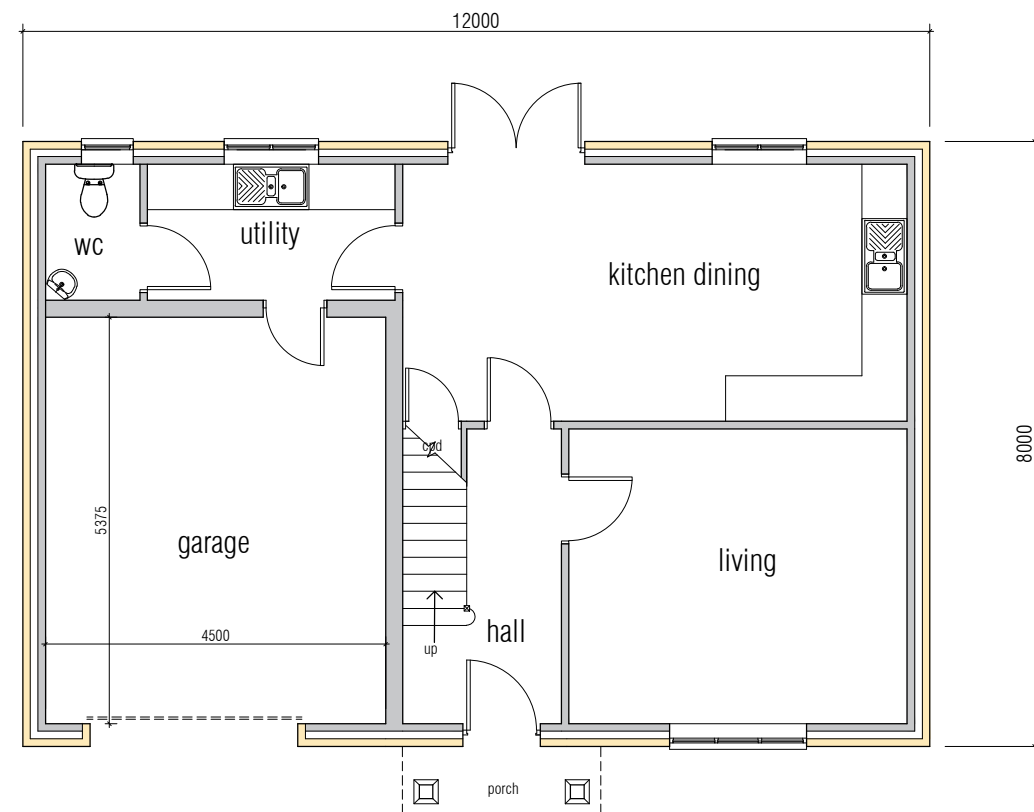
ground floor layout - plots 2 & 3
