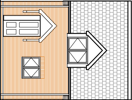
PLOT B SOUTH ELEVATION
