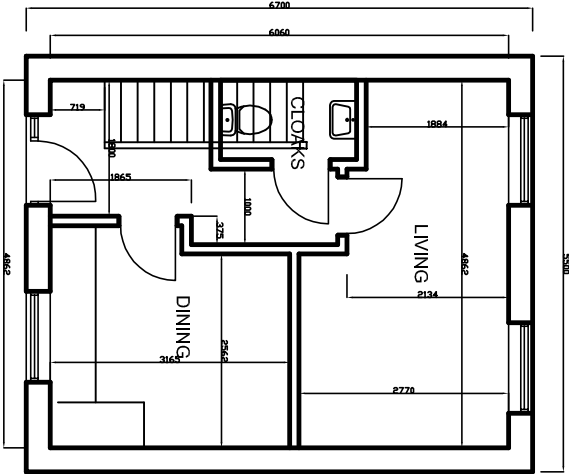
PLOT B FIRST FLOOR PLAN
