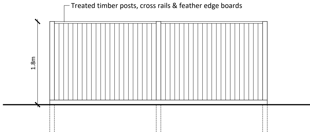
1.8m high close boarded fence
