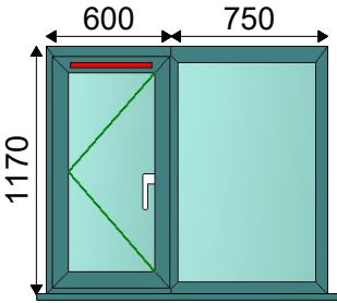
1 - 1350w x 1170h (Basic Frame Size) 1 - 1350w x 1200h, 30mm Cill Viewed Outside
