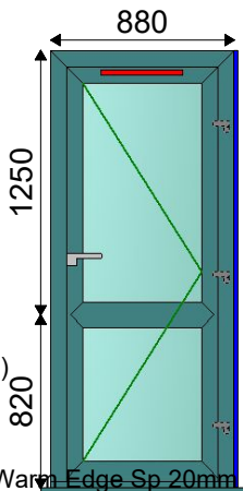
1 - 880w x 2070h (Basic Frame Size) 1 - 900w x 2100h, 30mm Cill Viewed Outside
