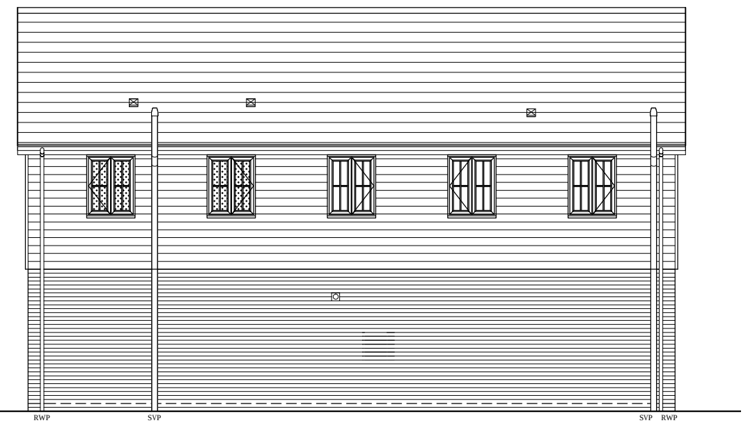
REAR ELEVATION
