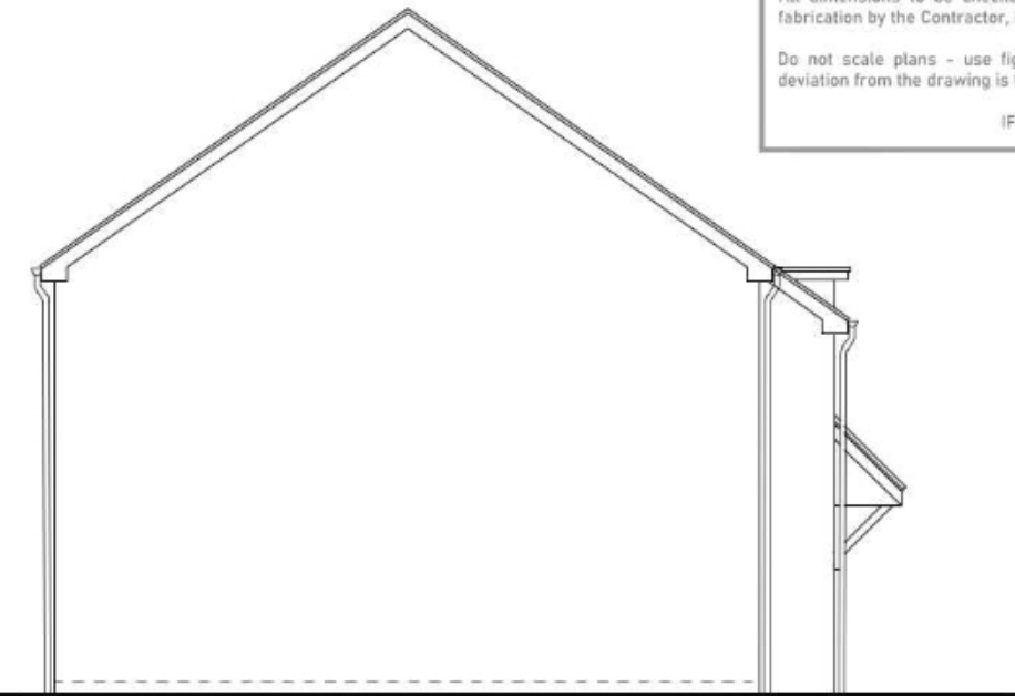
Side Elevation
