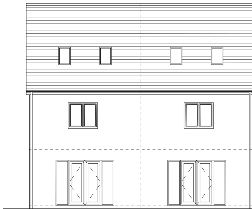
Rear Elevation
