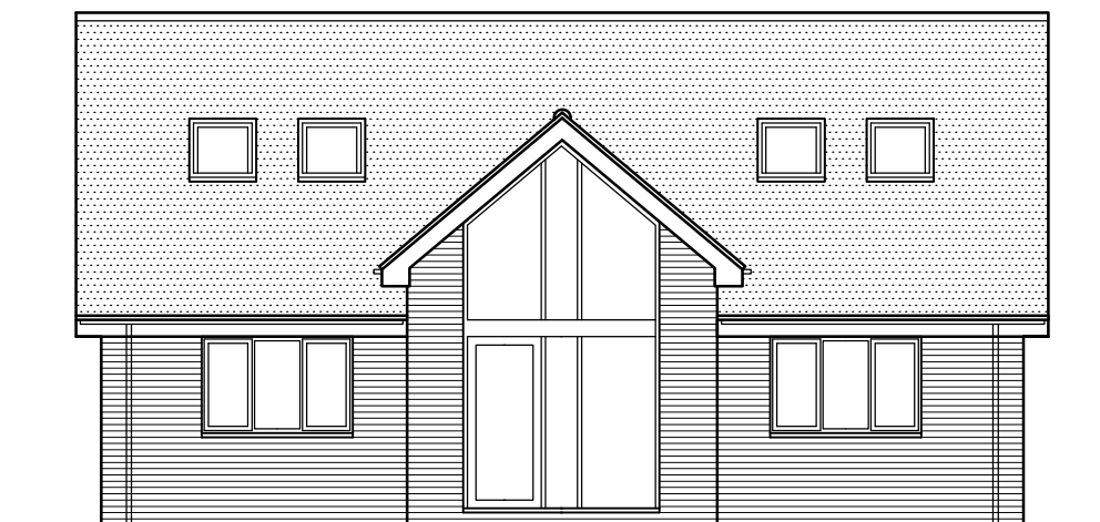
SOUTH EAST
