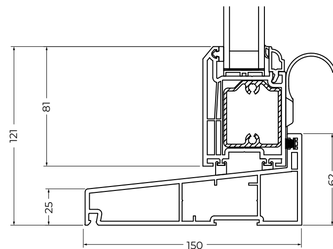
25mm standard flush cill
