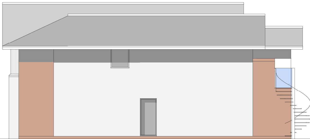
NORTH ELEVATION
