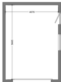
GARAGE FLOOR PLAN
