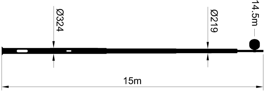
DETAIL OF 15m STEEL MONOPOLE
