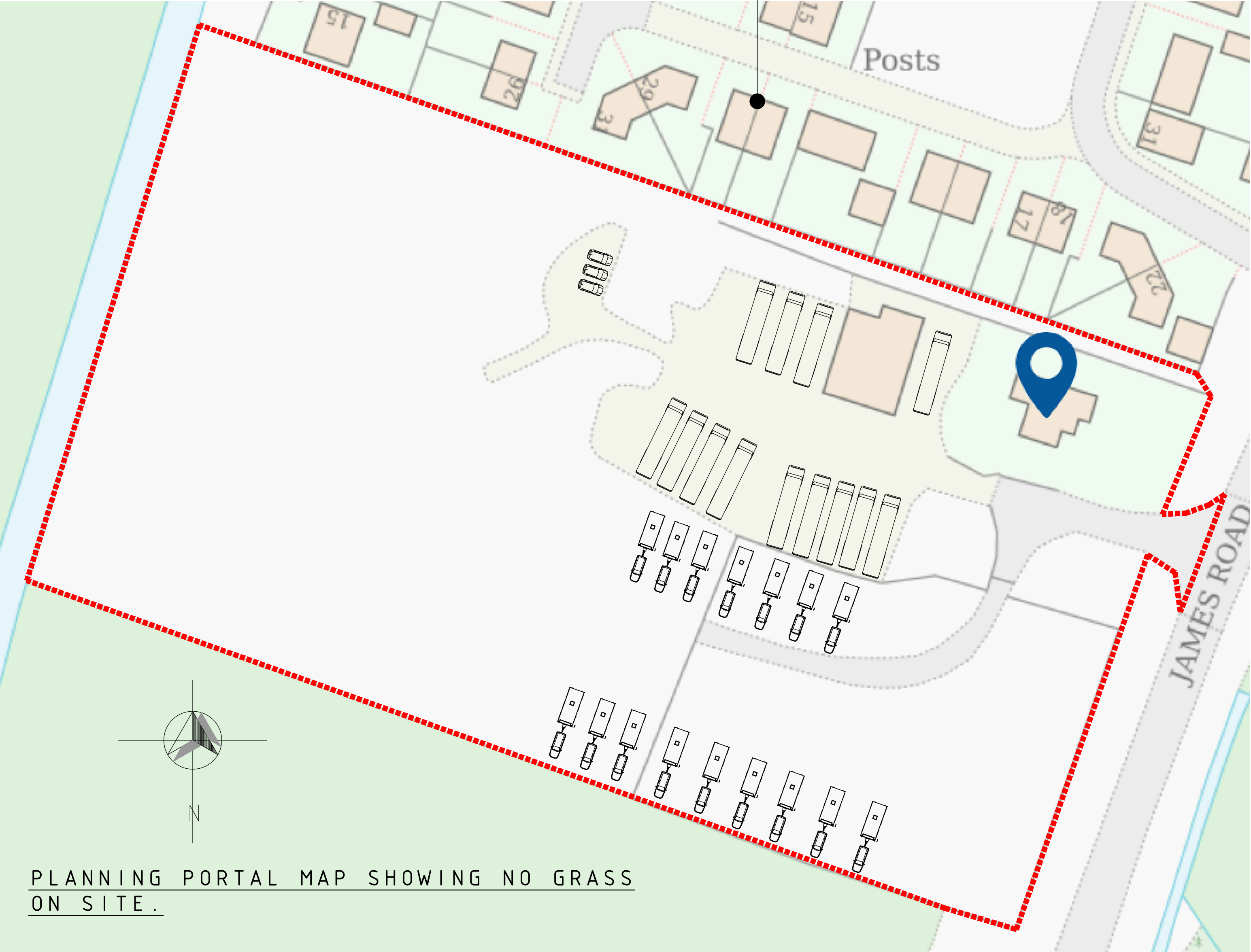
PRE-EXISTING BLOCK PLAN SCALE 1:500
