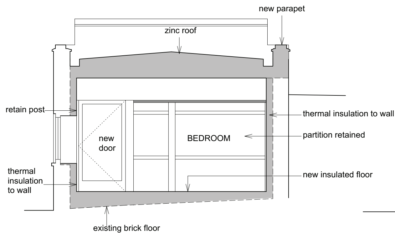
01 214 Proposed Section L-L 1:50@A3
