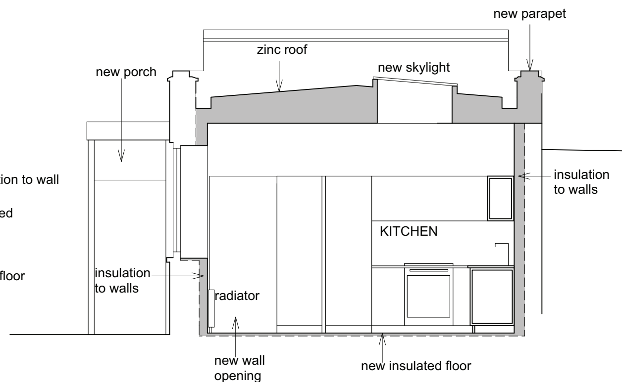
02 214 Proposed Section K-K 1:50@A3
