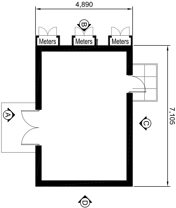
Typical DNO 33kV GRP Switchroom Plan 1:100
