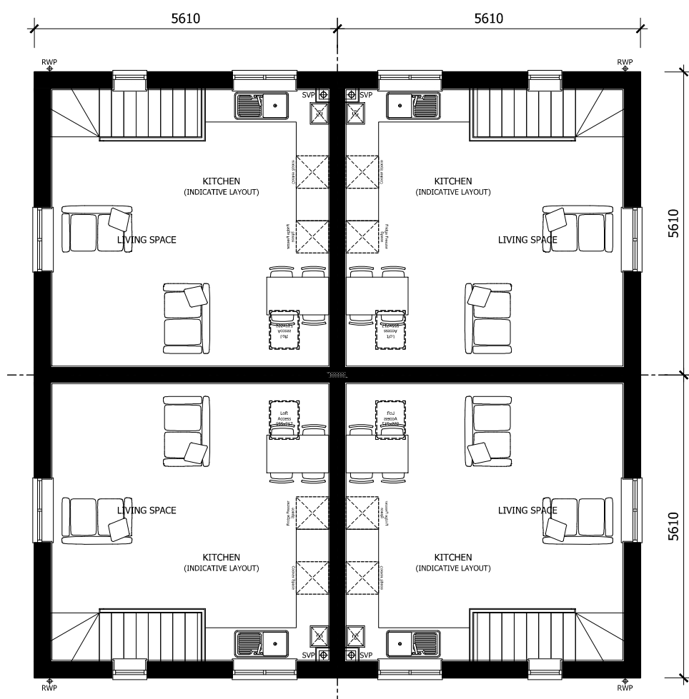
FIRST FLOOR
