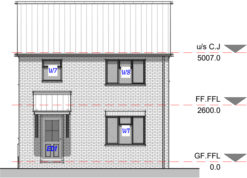
Elevation 01 - Front 1 : 100
