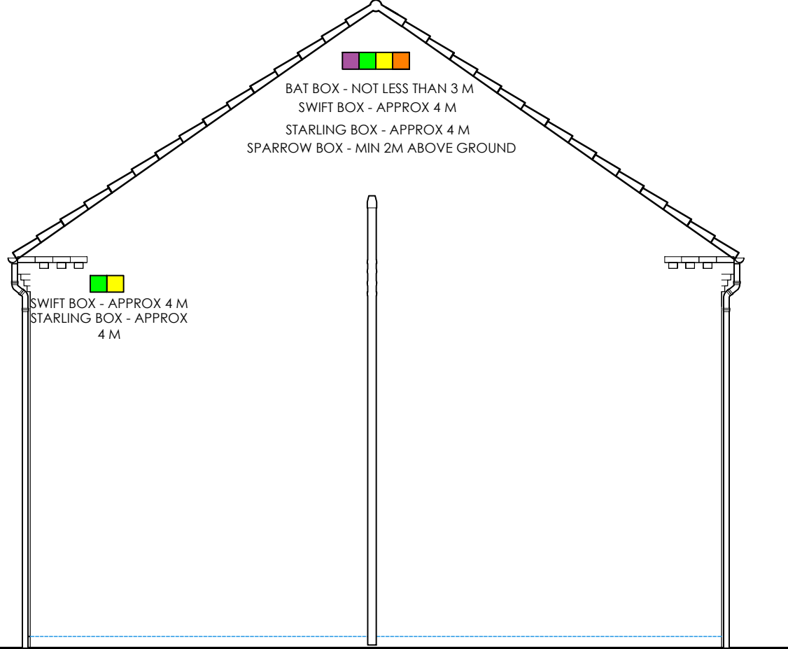
INDICATIVE SIDE ELEVATION
