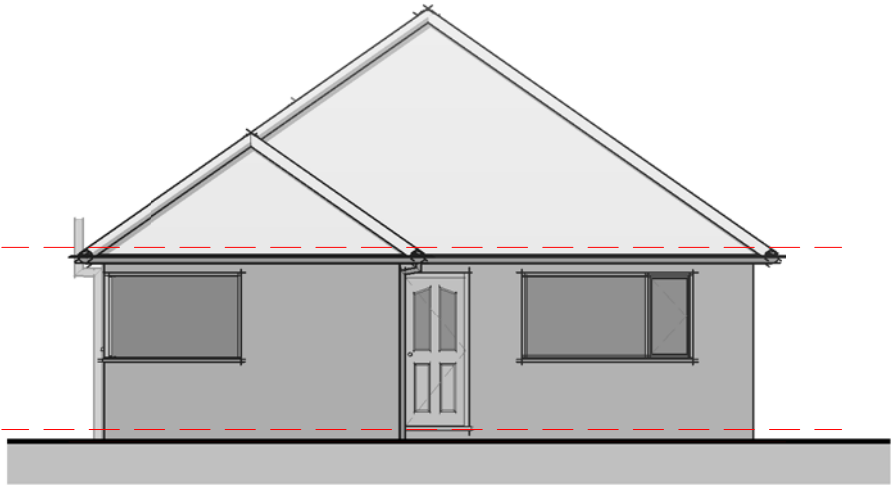
Elevation 01 - Front 1 : 100
