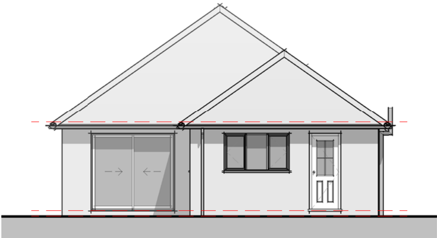
Elevation 03 - Rear 1 : 100
