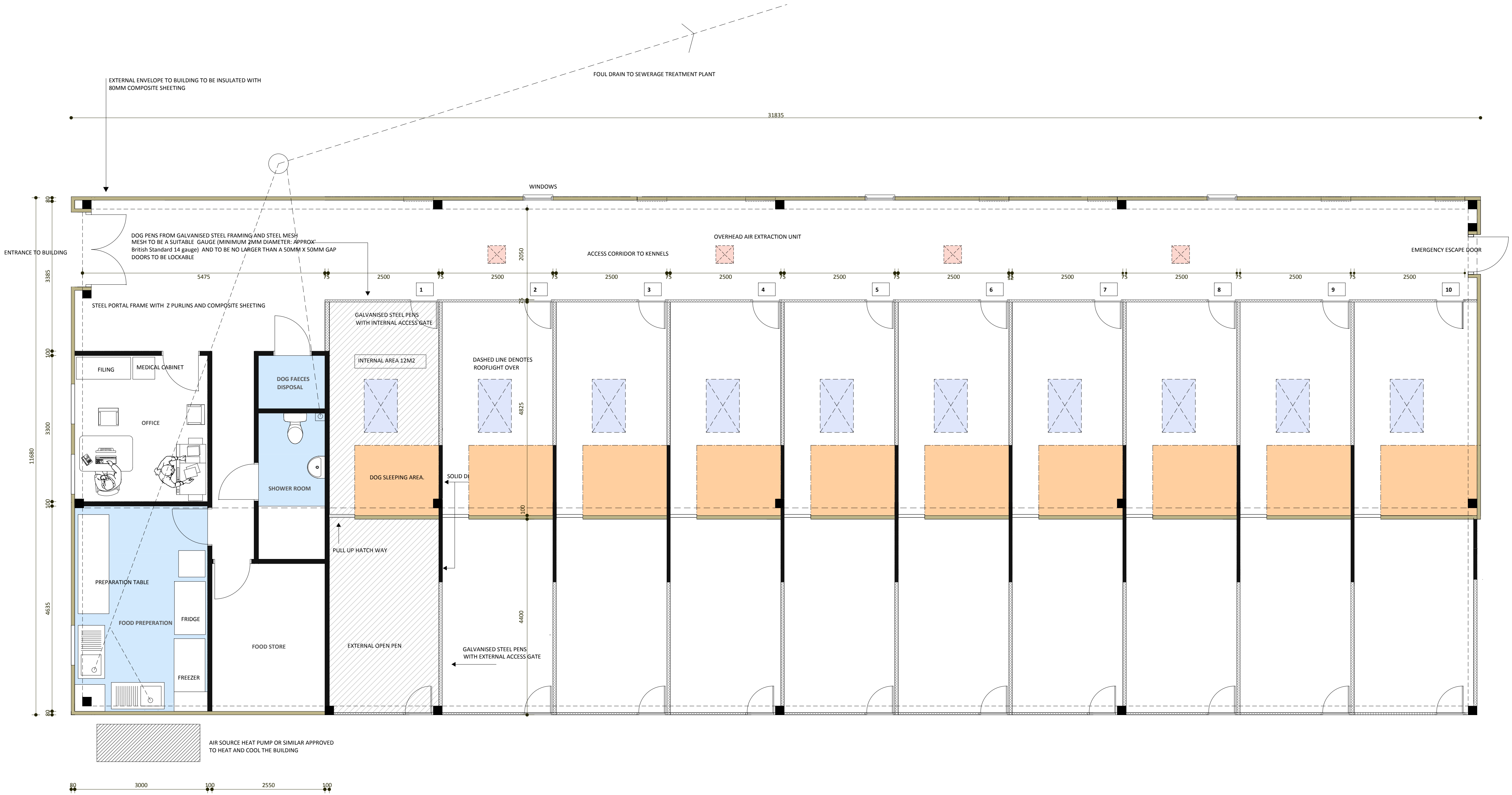
PLAN OF PROPOSED DOG KENNELS
