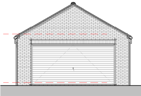
Elevation 01 – Front 1 : 100
