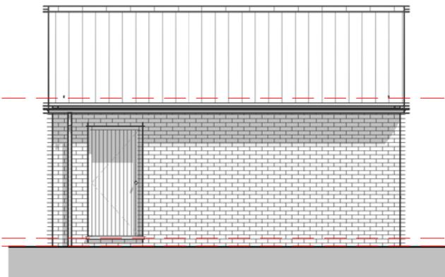
Elevation 04 – Left 1 : 100
