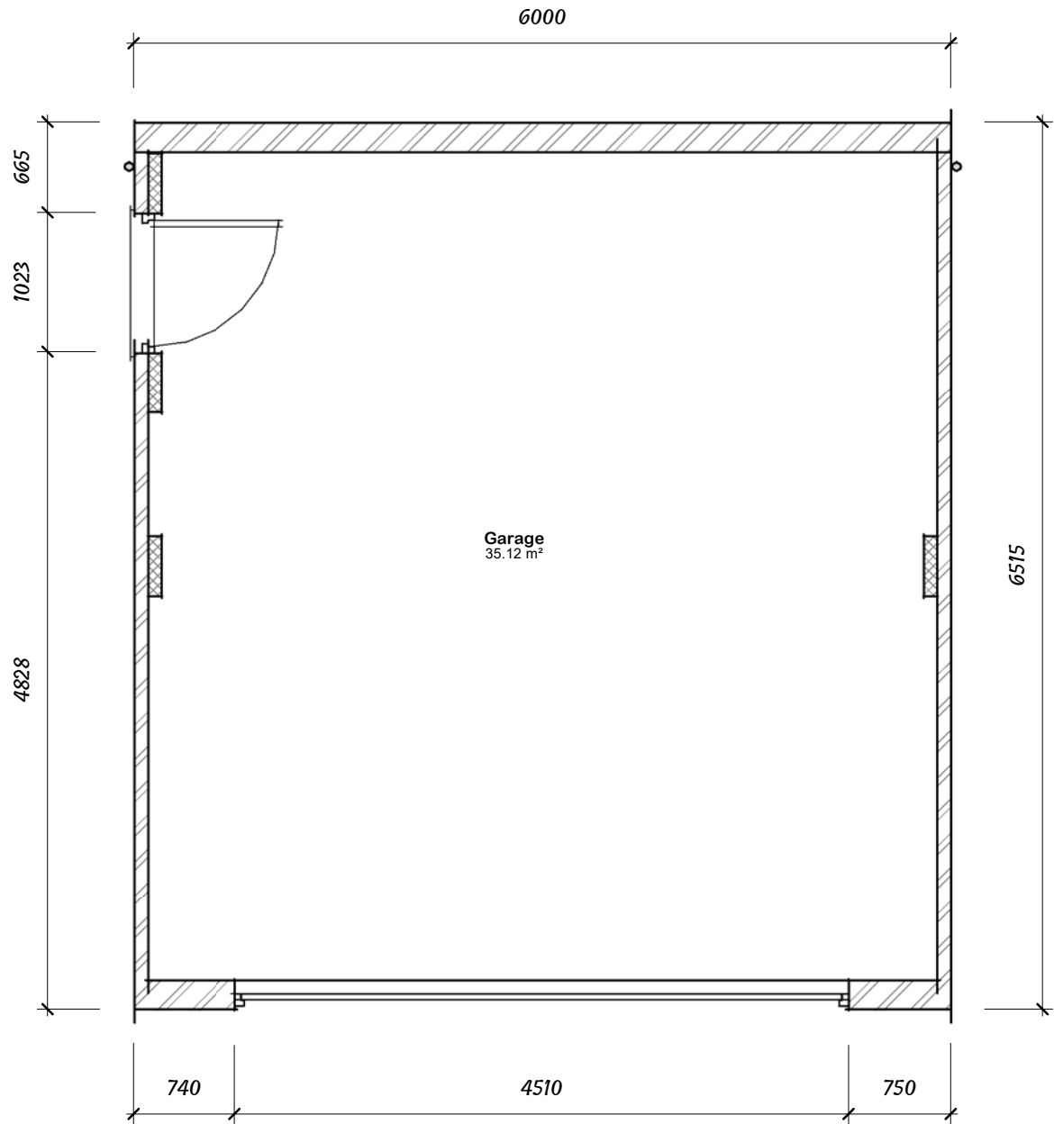
Plan 01 – Ground 1 : 50
