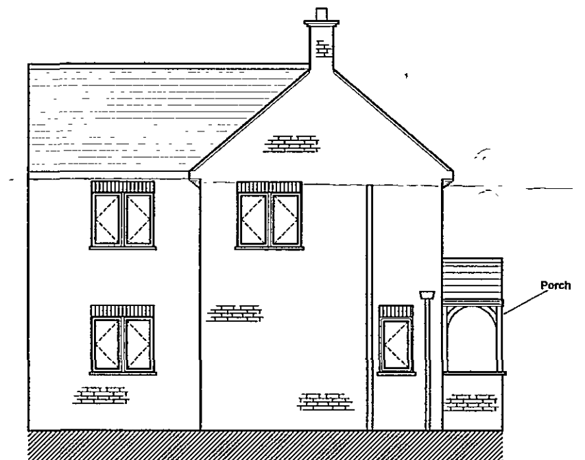
WEST ELEVATION
